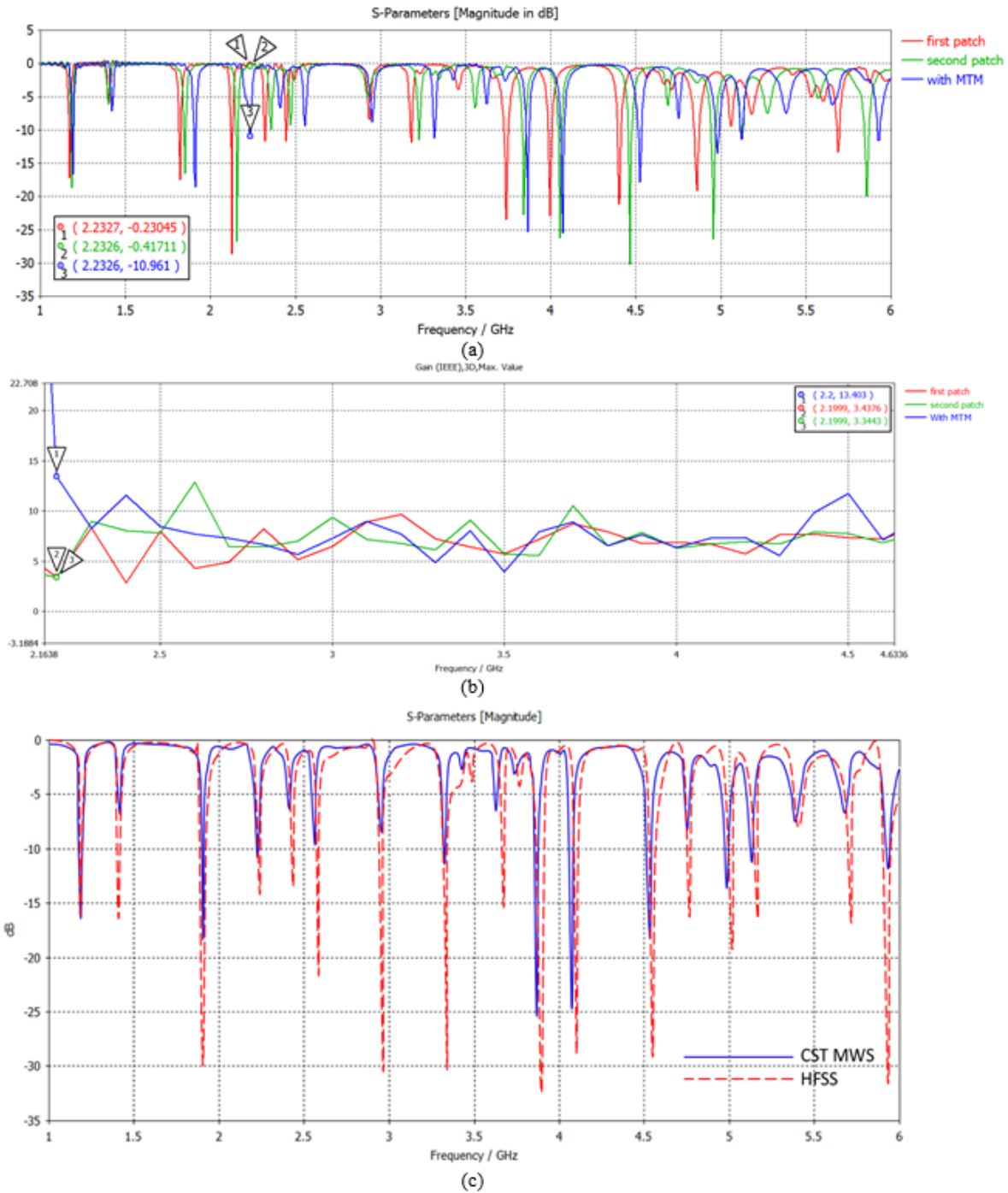
Figure 5: The simulated results of the proposed antenna (a): reflection coefficient of three stages of design (b): gain of three stages of design (c): comparison of the reflection coefficient using CST and HFSS.
