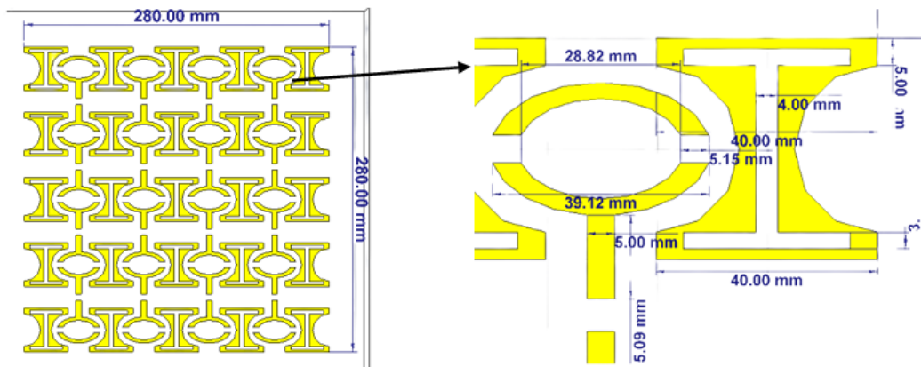
Figure 3: The MTM design structure.
