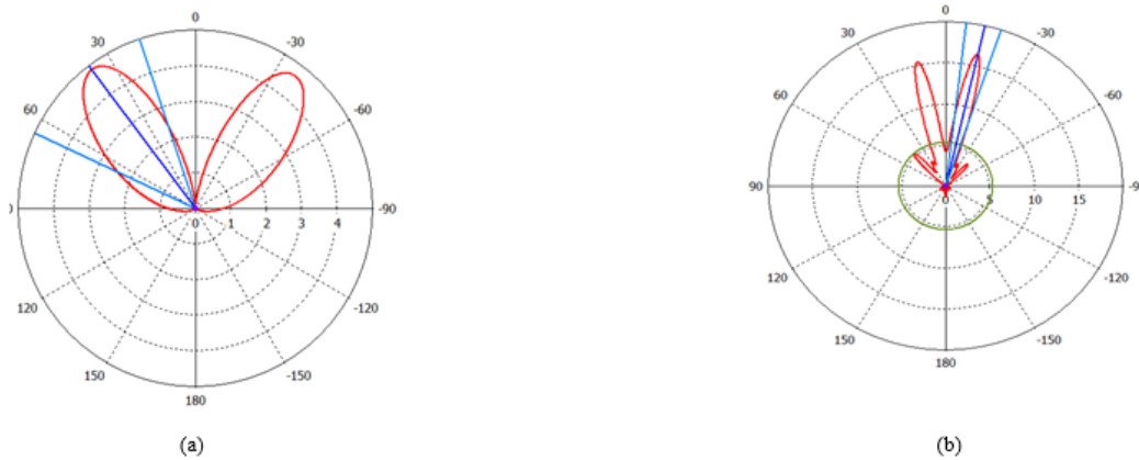
Figure 9: The radiation pattern of beam splitting with MTM and supersaturate (a) at 1.9 GHz (b) at 5.9 GHz.
