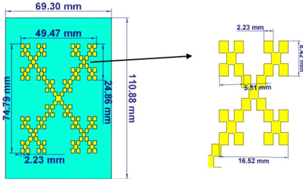
Figure 2: The supersaturate design structure.
