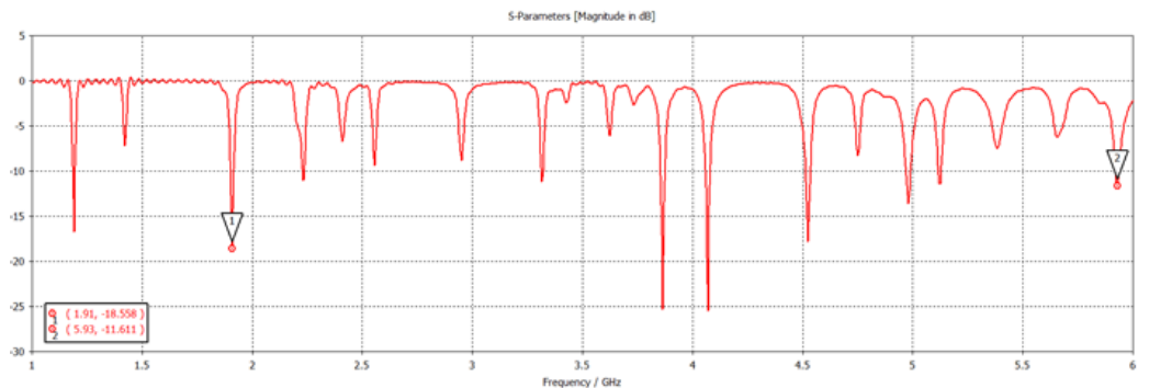
Figure 8: The reflection coefficient of the beam splitting at 1.9 and 5.9 GHz.
