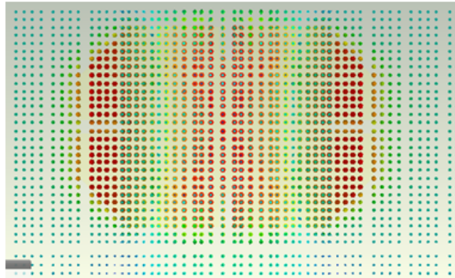
Figure 7: Current distribution result of the proposed antenna at 2.2 GHz.
