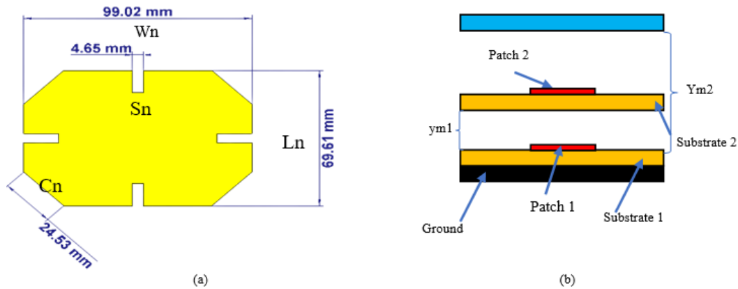
Figure 1: The structure of the antenna (a): patch antenna geometry (b): Schematic view of an antenna.
