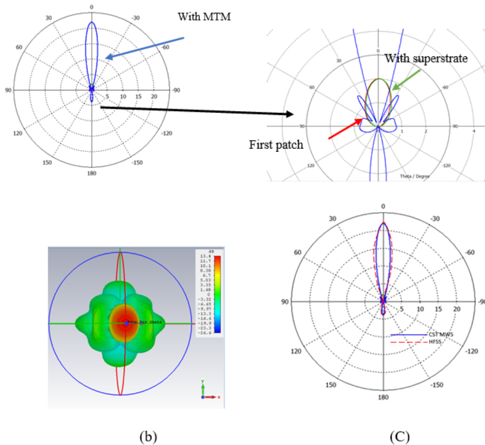
Figure 6: Radiation pattern results of the proposed antenna at 2.2 GHz (a): 2D dimensions (b): 3D dimensions (c): with HFSS program.
