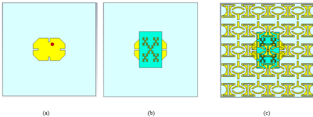
Figure 4: The final structure of the proposed antenna design (a): step 1 (b): step 2 (c): step3.
